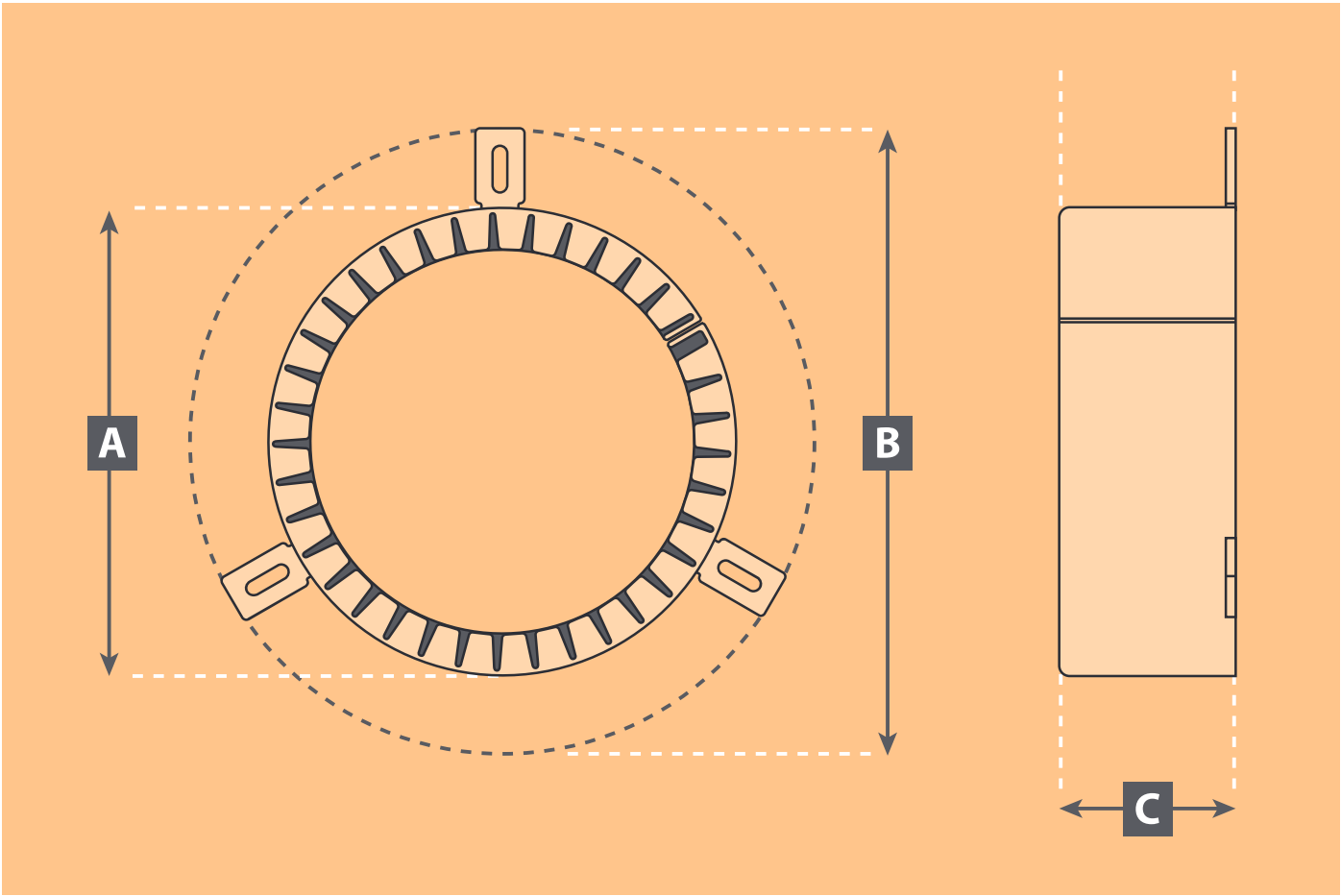
Firebreak FX300 Pipe Collar dimensions (nominal) and packaging data
